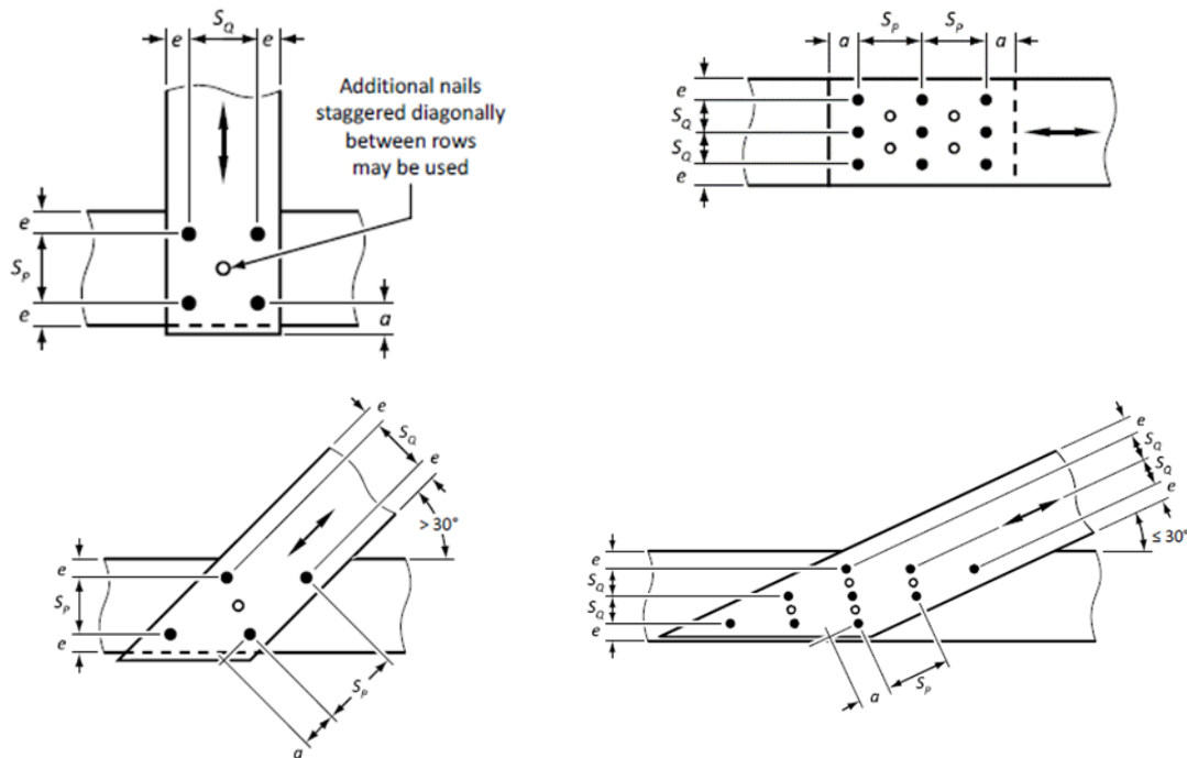
Figure 2. Example Diagrams Illustrating Fastener Spacings 10
