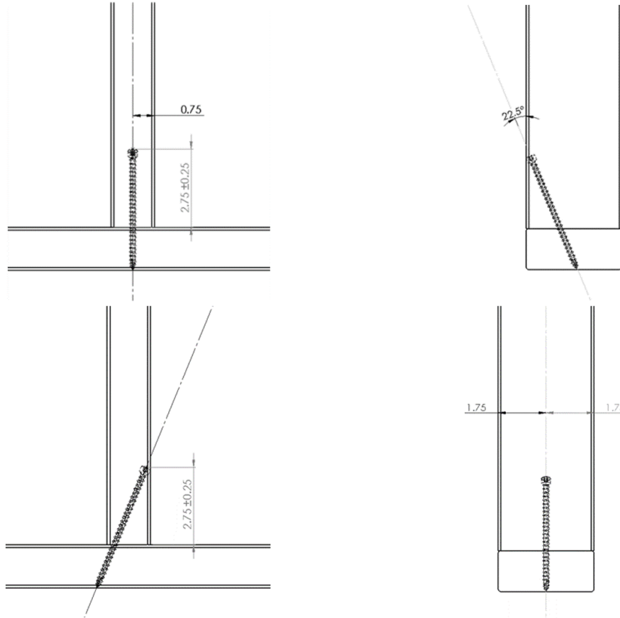
Figure 21. Stud to Bottom Plate – 22.5° (Angle), One 4½" TRX Truss Screw Option
