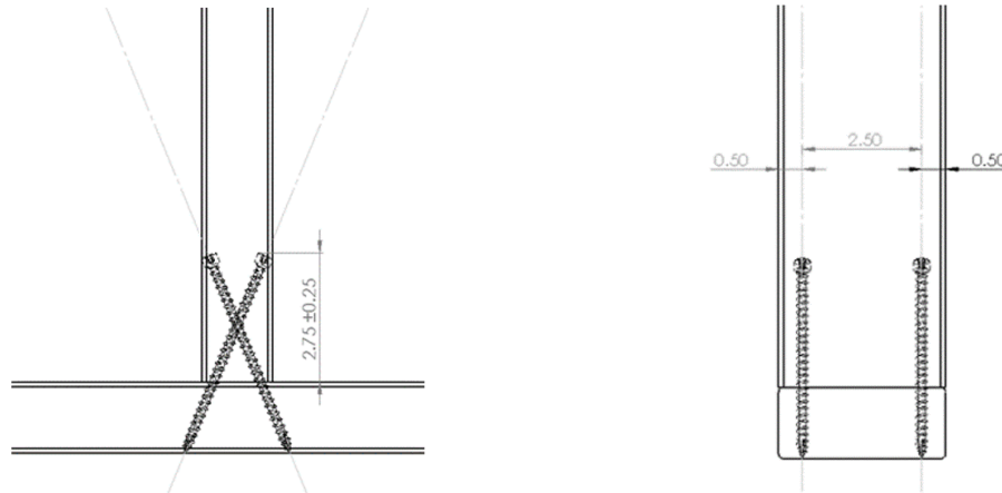
Figure 22. Stud to Bottom Plate – 22.5° (Angle), Two 4 \frac{1}{2} " TRX Truss Screws Install Option
