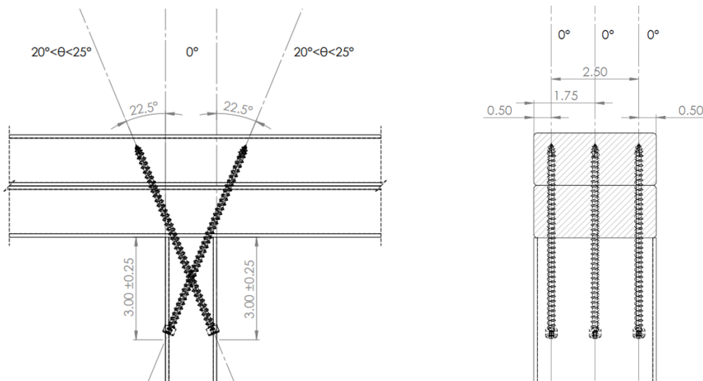
Figure 10. Stud to Top Plate – 22.5° (Angle), Three 6" TRX Truss Screws Install Option
