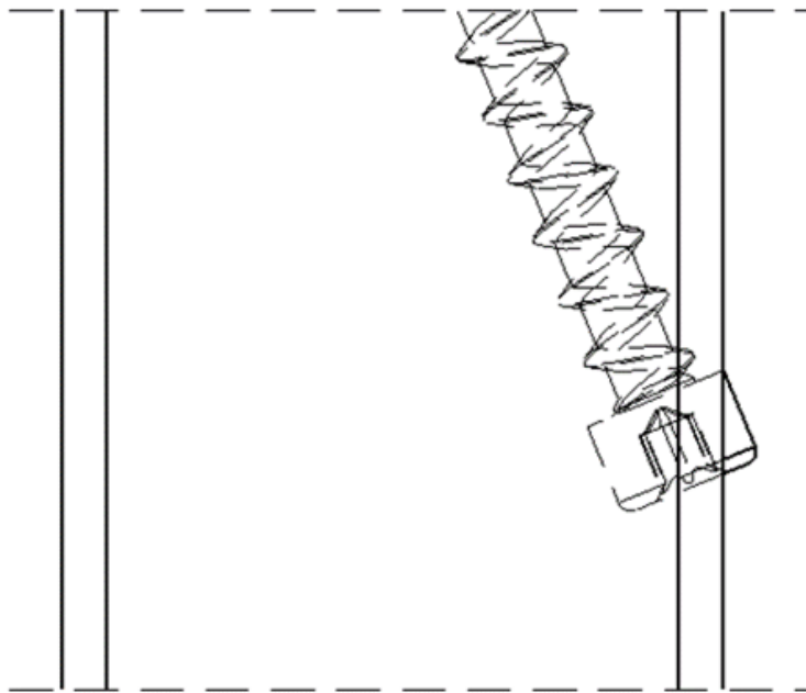
Figure 25. Diagram Showing Fastener Head Fully Bearing Against Stud
