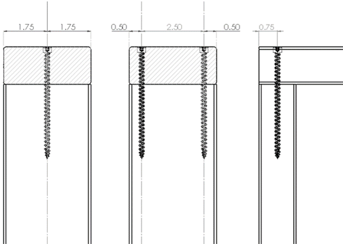
Figure 15. Stud to Top Plate – 0° (Perpendicular) Install Options
