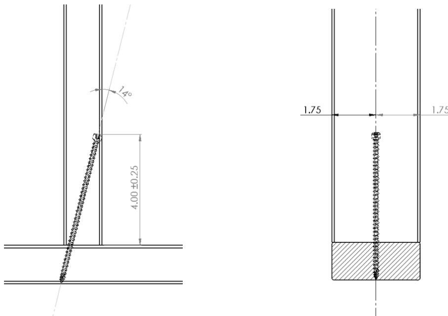
Figure 17. Stud to Bottom Plate – 14° (Angle), One 6" TRX Truss Screw Option
