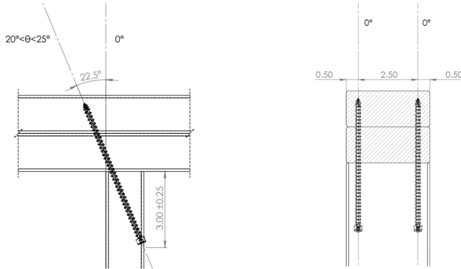
Figure 9. Stud to Top Plate – 22.5° (Angle), Two 6" TRX Truss Screws Install Option
