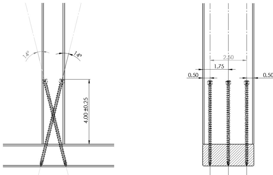
Figure 19. Stud to Bottom Plate – 4°-14° (Angle), Three 6" TRX Truss Screws Install Option
