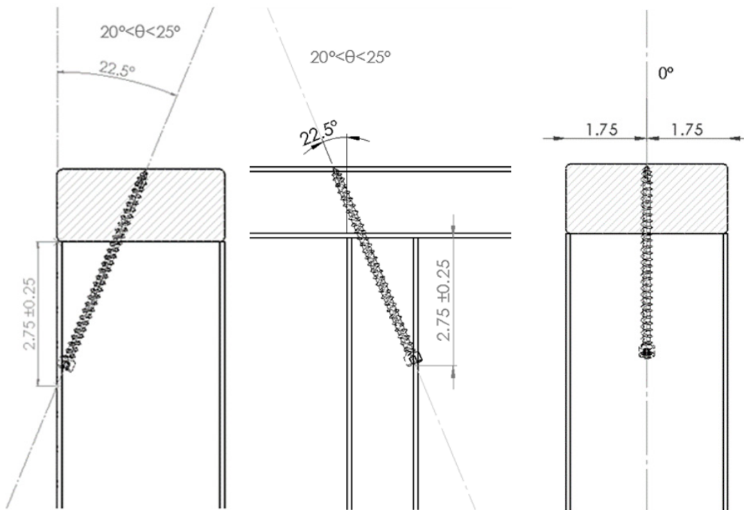
Figure 12. Stud to Top Plate – 22.5° (Angle), One 4½" TRX Truss Screw Options
