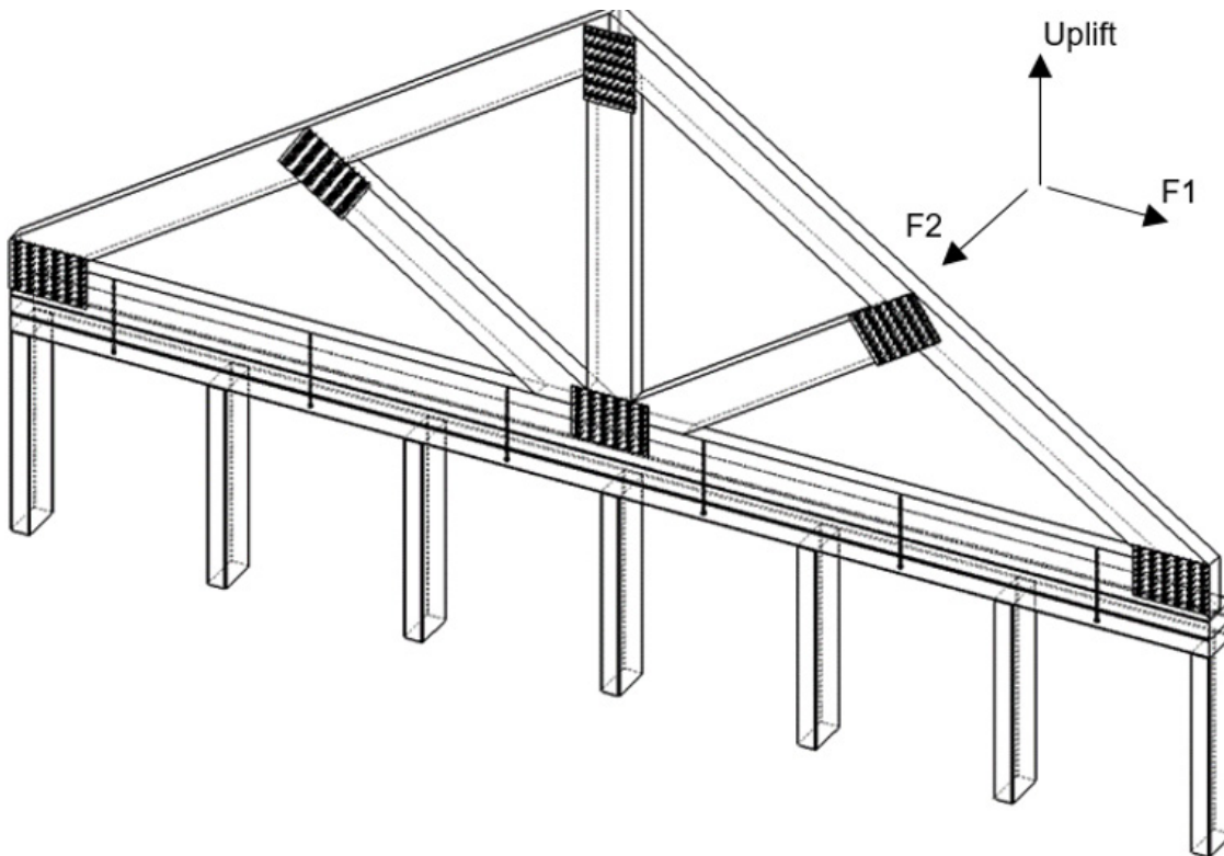
Figure 6. Gable End Truss to Top Plate - Uplift and Lateral Load (F1 and F2) Directions
