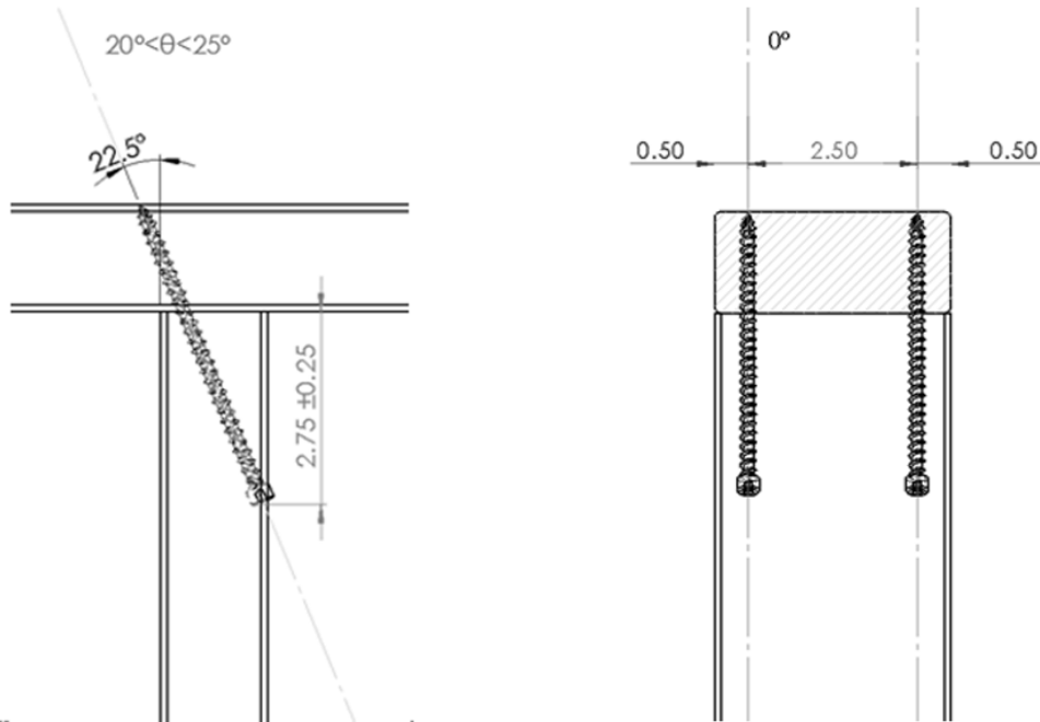
Figure 13. Stud to Top Plate – 22.5° (Angle), Two 4½" TRX Truss Screws Install Option
