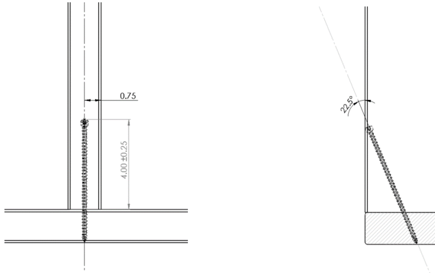
Figure 16. Stud to Bottom Plate – 22.5° (Angle), One 6" TRX Truss Screw Option
