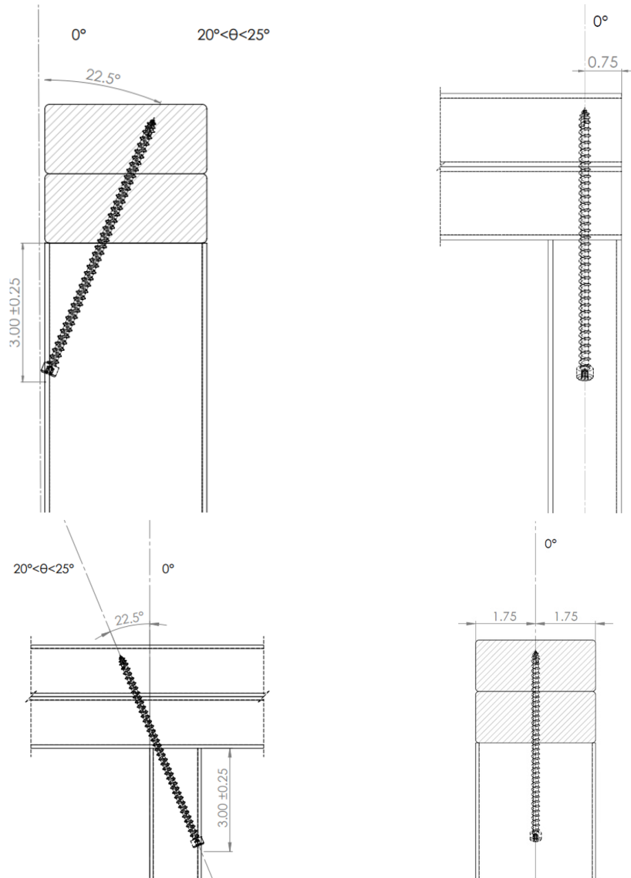
Figure 8. Stud to Top Plate – 22.5° (Angle), One 6" TRX Truss Screw Options
