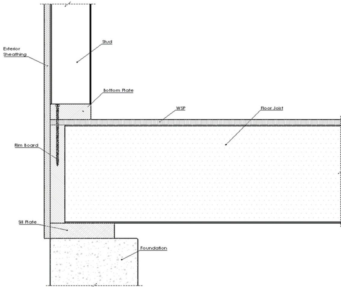
Figure 24. Fastener in Bottom Plate to Rim Board Connection
