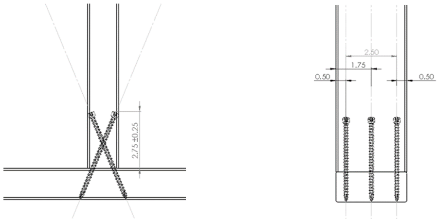
Figure 23. Stud to Bottom Plate – 22.5° (Angle), Three 4 \frac{1}{2} " TRX Truss Screws Install Option
