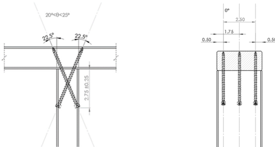
Figure 14. Stud to Top Plate – 22.5° (Angle), Three 4½" TRX Truss Screws Install Option
