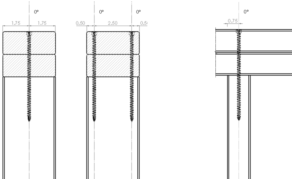
Figure 11. Stud to Top Plate – 0° (Perpendicular) Install Options
