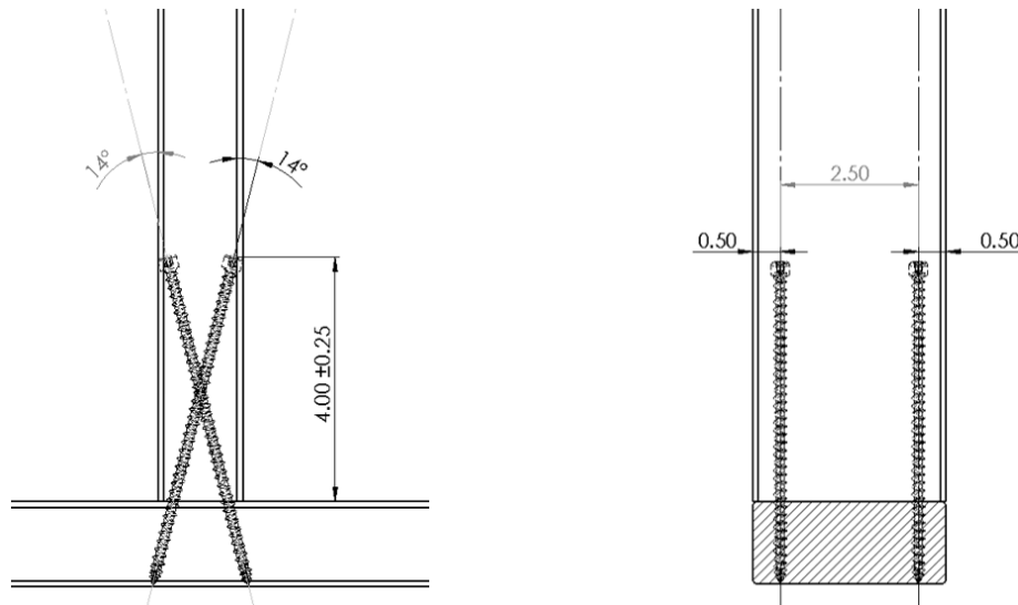
Figure 18. Stud to Bottom Plate – 4°-14° (Angle), Two 6" TRX Truss Screws Install Option
