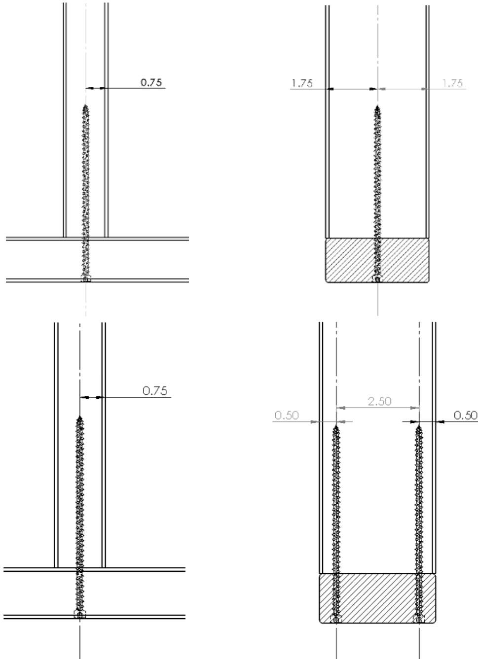
Figure 20. Stud to Bottom Plate – 0° (Perpendicular) Install Options
